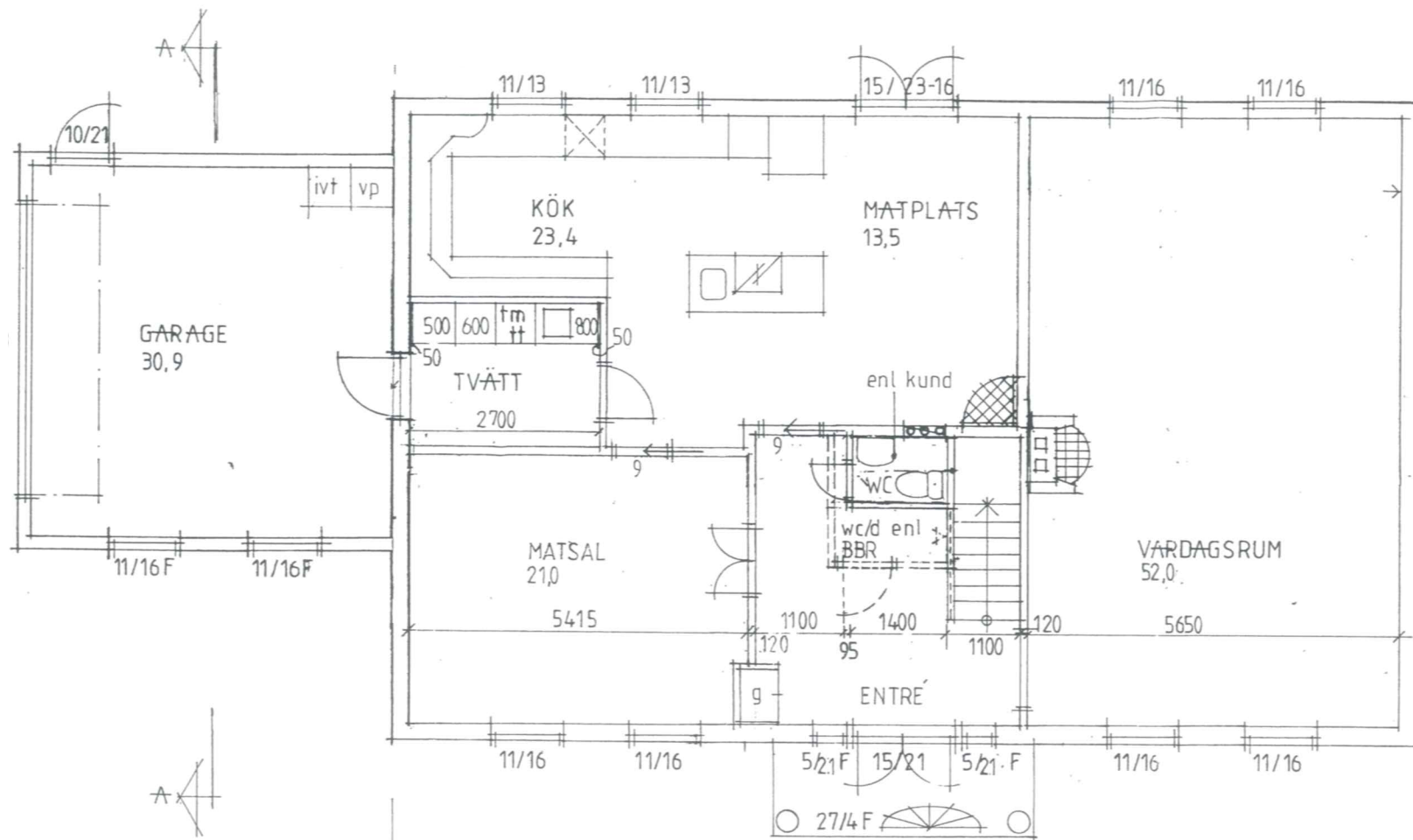
BOTTENPLAN BOA = 138,0 m 2 + 30,9 m 2
